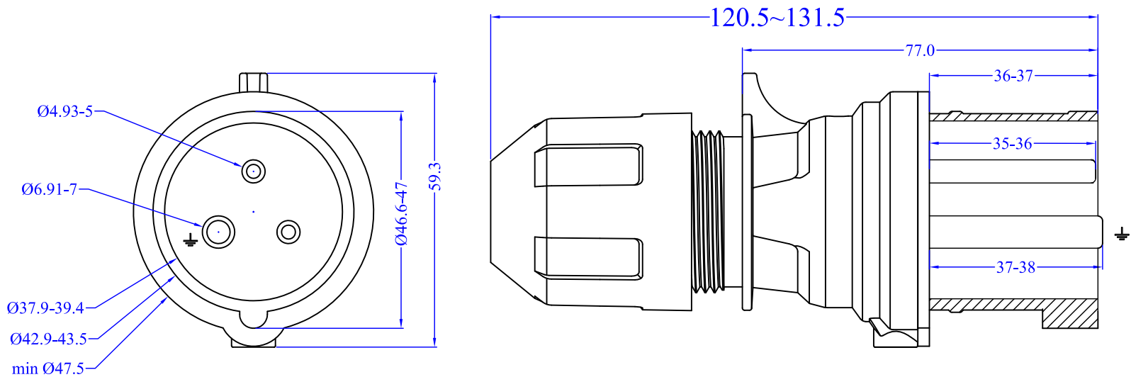
CEE Plug 16A-4h/100-130~,2P+E,IP44 H05VV-F/H07RN-F 3G1.5~4.0mm 2 EN60309
